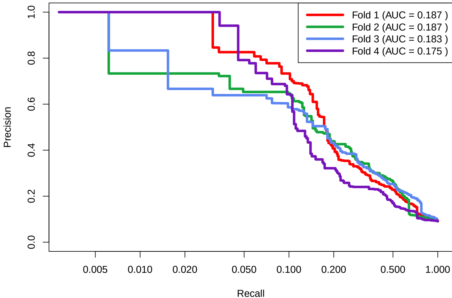
SPELL All Datasets: 430x50x20x10x1 Training
